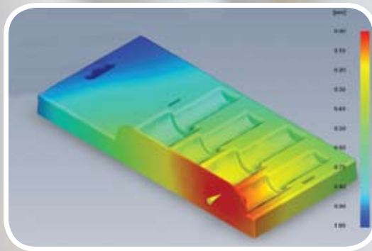
Omega Plastics utilizes its state-of-the-art Flow Analysis Program to ensure proper filling that detects potential problems before tooling is produced.
